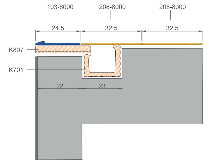
Tünel Sistem Detay-2 / Tunnel System Detail-2
